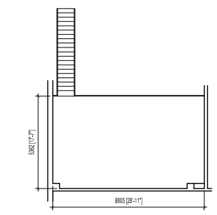
MEZZANINE AREA 1
